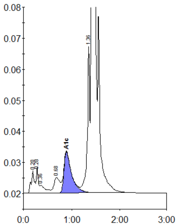
Peak table - ID: 10615484
